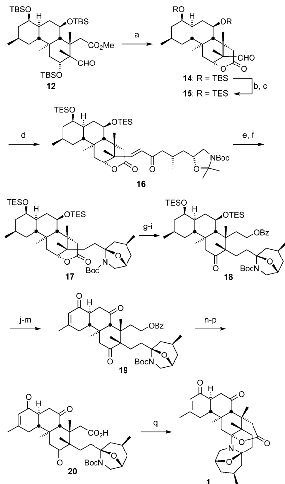
Scheme 4. Completion of the total synthesis of (–)-norzoanthamine ( 1 ). Reagents and conditions: a) TBAF, \text{THF} , 0^\circ\text{C} –RT, quant.; b) aq. HF (4 N), \text{CH}_3\text{CN} , RT, quant.; c) \text{TESCl} , imidazole, \text{CH}_2\text{Cl}_2 , RT, 76%; d) 6 , \text{LiCl} , i\text{Pr}_2\text{NEt} , \text{CH}_3\text{CN} , 60^\circ\text{C} , 67% (94% based on the recovered starting material); e) \text{H}_2 , \text{Pd/C} , \text{EtOH} , RT, 96%; f) \text{AcOH} , \text{H}_2\text{O} , 50^\circ\text{C} , 56%; g) \text{AlH}_3 – \text{EtNMe}_2 , toluene, 50^\circ\text{C} , 59%; h) \text{BzCl} , \text{NEt}_3 , \text{CH}_2\text{Cl}_2 , 0^\circ\text{C} –RT, 88%; i) \text{DMP} , \text{CH}_2\text{Cl}_2 , RT, quant.; j) aq. HF (0.5 N), \text{CH}_3\text{CN} , 0^\circ\text{C} –RT, 94%; k) \text{DMP} , \text{CH}_2\text{Cl}_2 , RT, quant.; l) \text{LHMDS} , \text{TMSCl} , \text{THF} , -78^\circ\text{C} ; m) cat. \text{Pd}(\text{OAc})_2 , \text{O}_2 , \text{DMSO} , 60^\circ\text{C} , 74% (over 2 steps); n) \text{K}_2\text{CO}_3 , \text{MeOH} , RT; o) \text{DMP} , \text{CH}_2\text{Cl}_2 , RT; p) \text{NaClO}_2 , \text{NaH}_2\text{PO}_4 , 2-methyl-2-butene, t\text{BuOH} , \text{H}_2\text{O} , RT, 66% (over 3 steps); q) \text{AcOH} , \text{H}_2\text{O} , 100^\circ\text{C} , 92%. \text{Bz} = benzoyl, \text{DMSO} = dimethyl sulfoxide, \text{LHMDS} = lithium hexamethyldisilazane, \text{TBAF} = tetra- n -butylammonium fluoride, \text{TES} = triethylsilyl.
