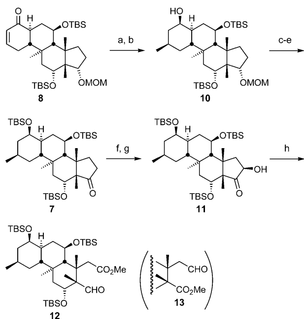
Scheme 3. Synthesis of formyl ester 12 . Reagents and conditions: a) \text{Me}_2\text{CuLi} , \text{Et}_2\text{O} , -78 – 0^\circ\text{C} , 91%; b) \text{NaBH}_4 , \text{MeOH} , 0^\circ\text{C} –RT, 79%; c) \text{TBSOTf} , 2,6-lutidine, \text{CH}_2\text{Cl}_2 , 0^\circ\text{C} –RT, 95%; d) B -bromocatecholborane, \text{CH}_2\text{Cl}_2 , -78^\circ\text{C} , 87%; e) \text{DMP} , \text{CH}_2\text{Cl}_2 , 0^\circ\text{C} –RT, quant.; f) n\text{BuLi} , \text{TMSCl} , \text{THF} , -78 – 0^\circ\text{C} ; g) \text{O}_3 , \text{CH}_2\text{Cl}_2 , \text{MeOH} , -78^\circ\text{C} , 79% (over 2 steps); h) \text{Pb}(\text{OAc})_4 , benzene, \text{MeOH} , 0^\circ\text{C} –RT, 77%. \text{DMP} = Dess–Martin periodinane, \text{Tf} = trifluoromethanesulfonyl, \text{TMS} = trimethylsilyl.
